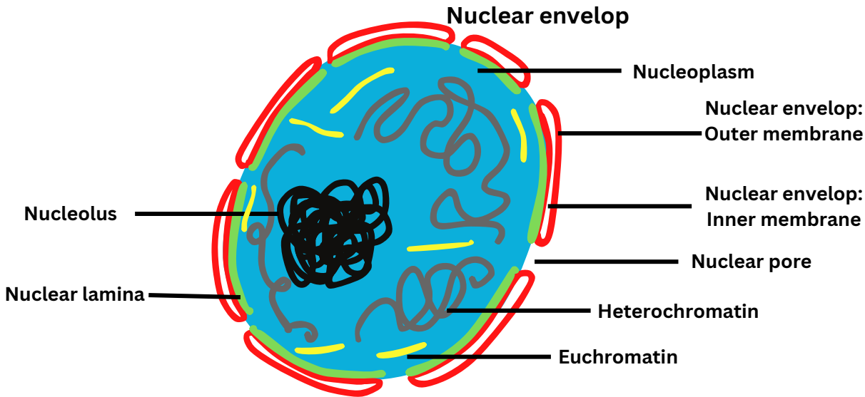
Simple diagram of Nucleus
